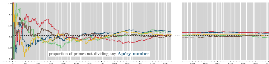
Figure 1: Proportion of primes (up to 10,000) not dividing the sequences (\delta) , (\alpha) , (\epsilon) , (\zeta) , (\gamma) , with the dotted line indicating e^{-1/2} . The Apéry sequence is plotted in blue. (We thank Arian Daneshvar for producing this plot.)
